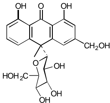
Fig 45. 10-(1',5'-anhydroglucosyl)-aloe-emodin-9-anthrone
